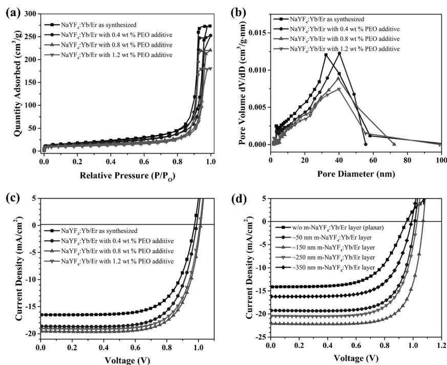
Figure 3. a) The nitrogen adsorption–desorption isotherms of NaYF 4 :Yb/Er mesoporous films and b) the corresponding pore-size distributions. c) The current density–voltage ( J – V ) characteristics of CH 3 NH 3 PbI 3 solar cells using NaYF 4 :Yb/Er mesoporous layers with varied ratios of PEO additives. d) The J – V characteristics of CH 3 NH 3 PbI 3 solar cells fabricated on different thicknesses of NaYF 4 :Yb/Er mesoporous layers.
