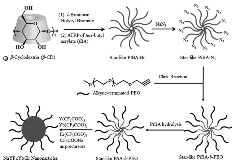
Figure 1. Scheme of the synthetic route to NaYF 4 :Yb/Er upconversion nanoparticles (UCNPs) by capitalizing on the double hydrophilic star-like poly(acrylic acid)- block -poly(ethylene oxide) (PAA- b -PEO) diblock copolymer as a nanoreactor.
